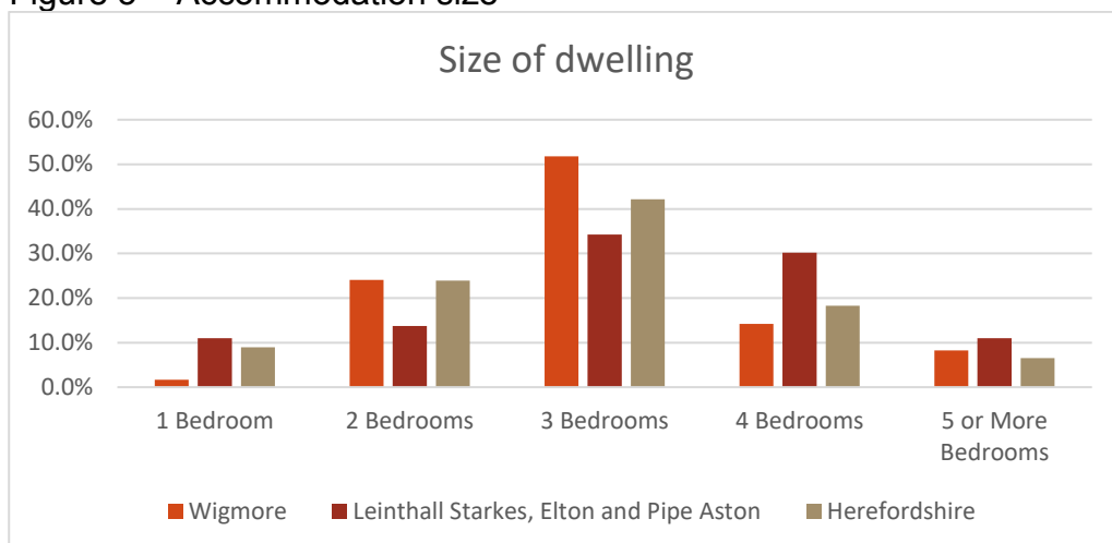
Figure 5 – Accommodation size
