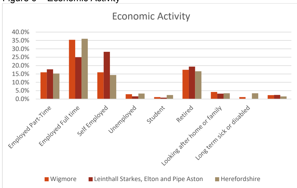
Figure 6 – Economic Activity
