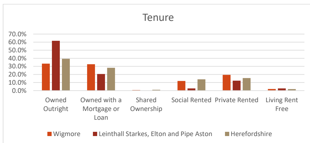
Figure 4 – Accommodation Tenure
