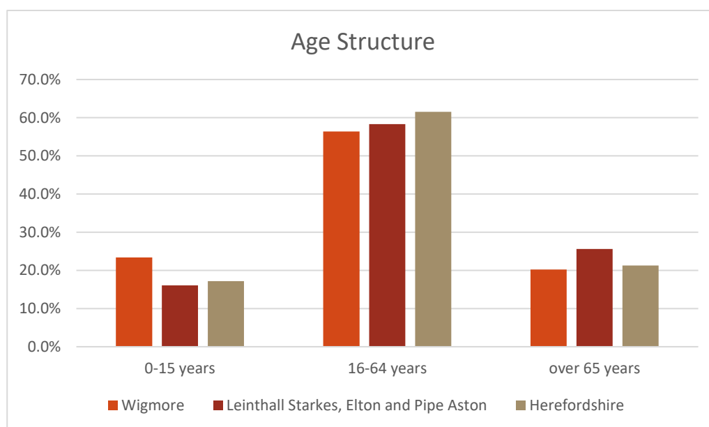
Figure 2 – Age Structure
