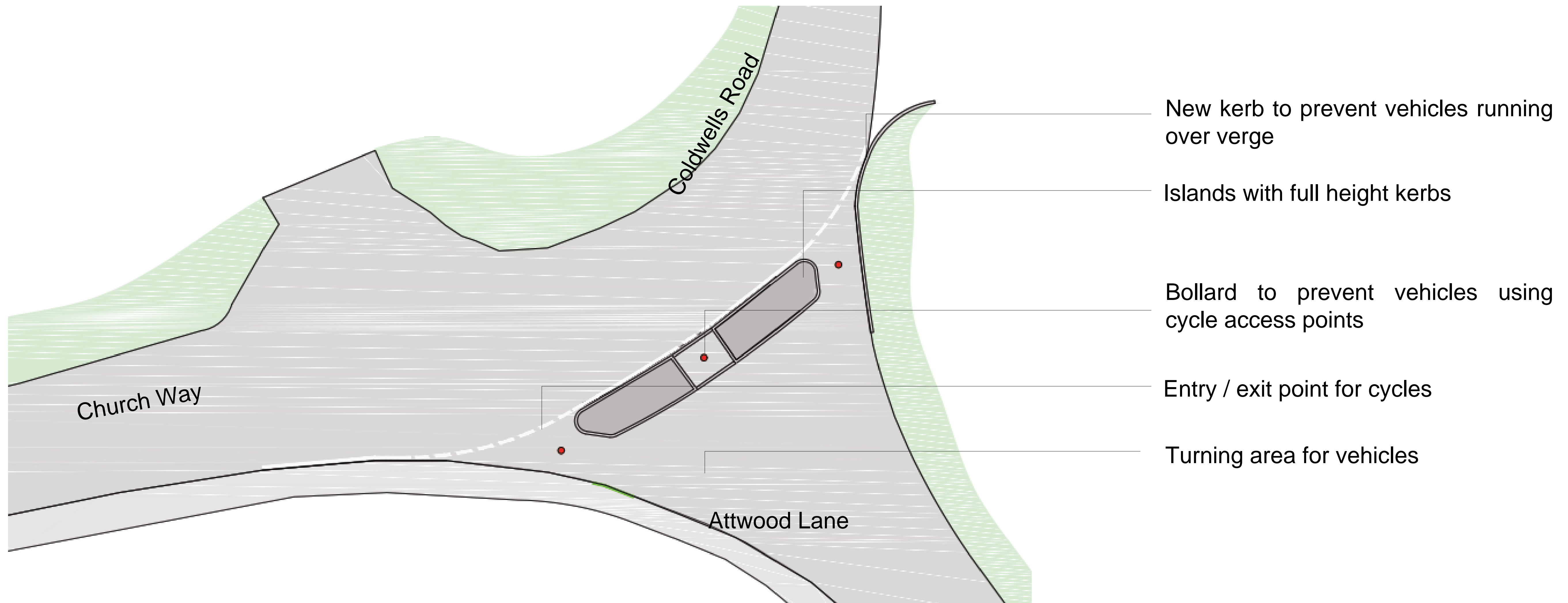
Layout of alterations at Atwood Lane, Church Way, Coldwells Road Junction
